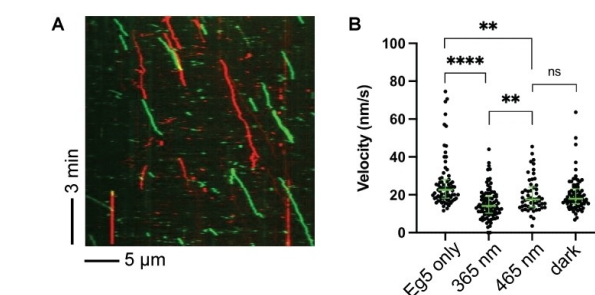
Figure 4. A) Overlaid kymographs of Eg5 only (green) and Eg5 with 3 μM pre-activated Azo-EMD (red) moving along microtubules. B) Velocities of Eg5 only (Eg5 only), Eg5 with 3 μM pre-activated Azo-EMD (365 nm), Eg5 with 3 μM Azo-EMD, pre-irradiated with 465 nm, and Eg5 with 3 μM dark adapted Azo-EMD (dark). The green bars represent the median with quartiles. Eg5 only: 22.6 [18.2, 28] nm s -1 ; 365 nm: 14.1 [10.2, 19.1] nm s -1 ; 465 nm: 17.6 [13.6, 24.0] nm s -1 ; Dark: 17.9 [15.3, 23.1] nm s -1 . Unpaired t -test were performed (****, p < 0.0001 ; **, p < 0.01 ; ns, p > 0.05 ).
