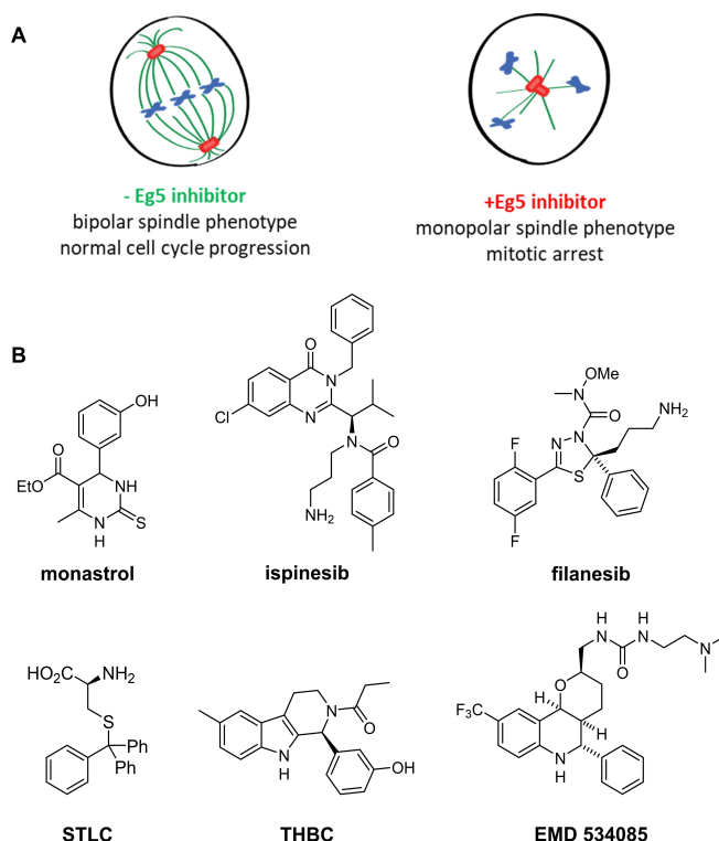
Figure 1. A) Eg5 is involved in the formation of the bipolar spindle during mitosis. When its function is inhibited, monopolar spindle formation is observed, which is followed by subsequent mitotic arrest. B) Structural diversity of allosteric Eg5 inhibitors.
